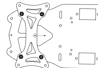
Wheel Base 250mm Setup
