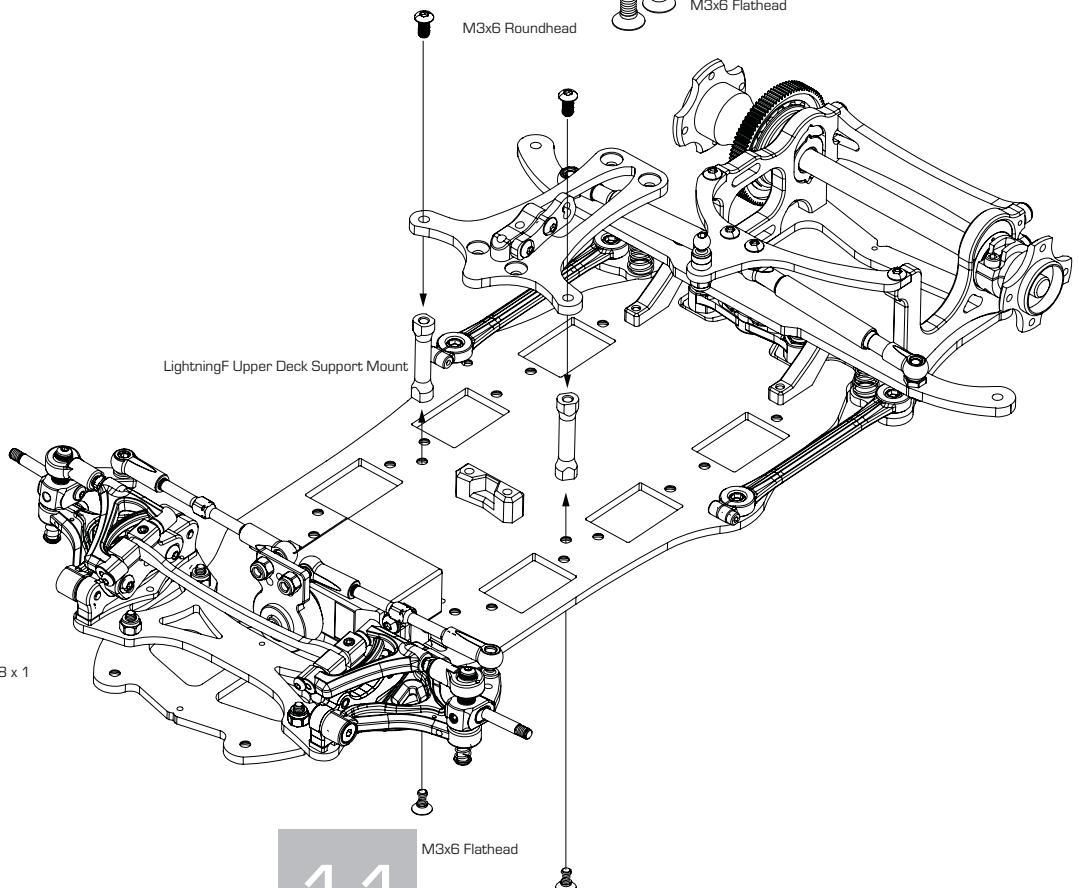
LightningF Upper Deck Support Mount B-02-VBC-5096 x 2
