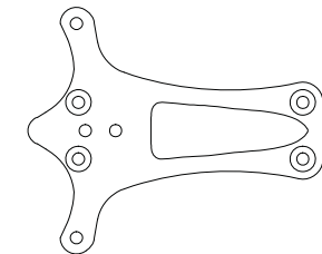
Lightning10 Graphite Front Shock Mount Plate A-01-P50208 x 1
