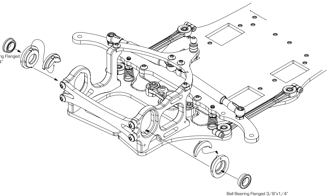
Lightning 12 Axle Height Adjuster D-05-VBC-0114
