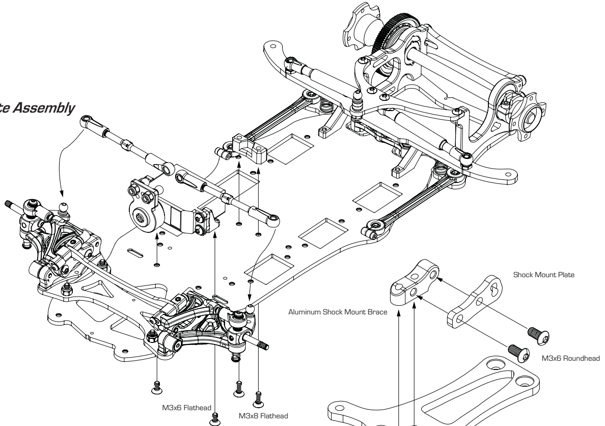
Lightning10 Graphite Front Shock Mount Plate A-01-P50208
