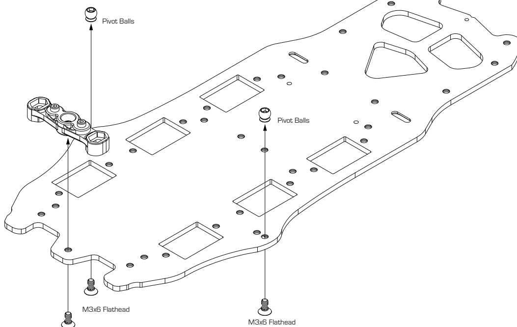
Pivot Brace Cover D-05-VBC-0101 x 1
