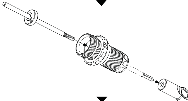
TBX Shock Ball End
