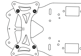
Wheel Base 253mm Setup
