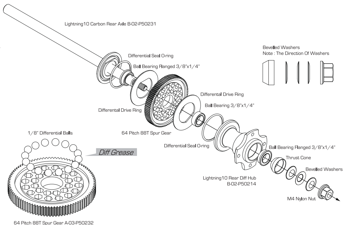
Ball Bearing 3/8"x1/4" C-02-BB-3B14 x 1
