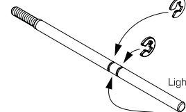
M1.5 E-Clip
