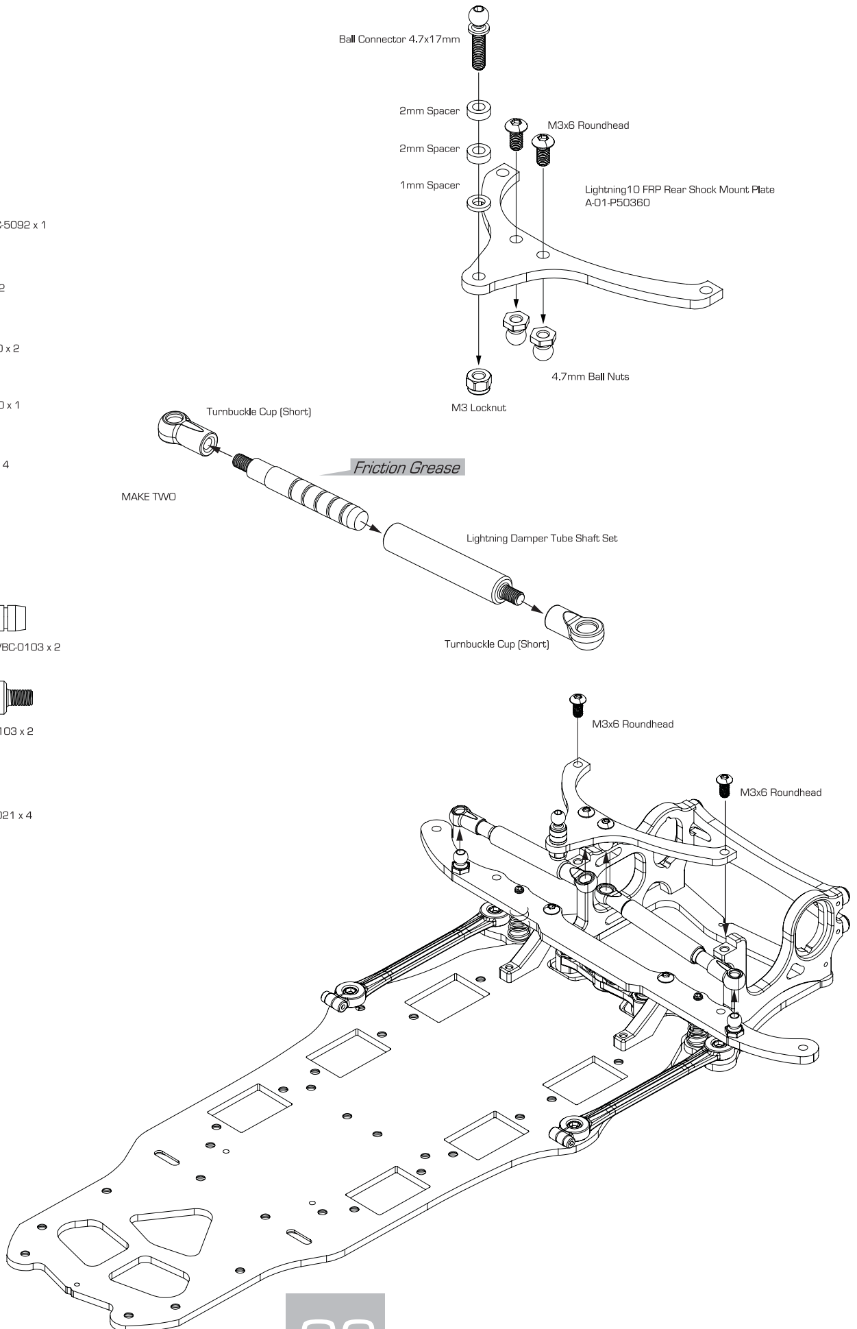
4.7mm Ball Nuts B-02-VBC-5020 x 2
