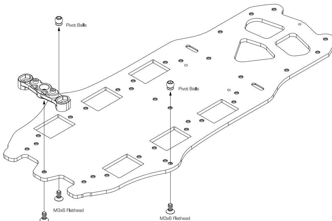
Pivot Brace Cover D-05-VBC-0101 x 1
