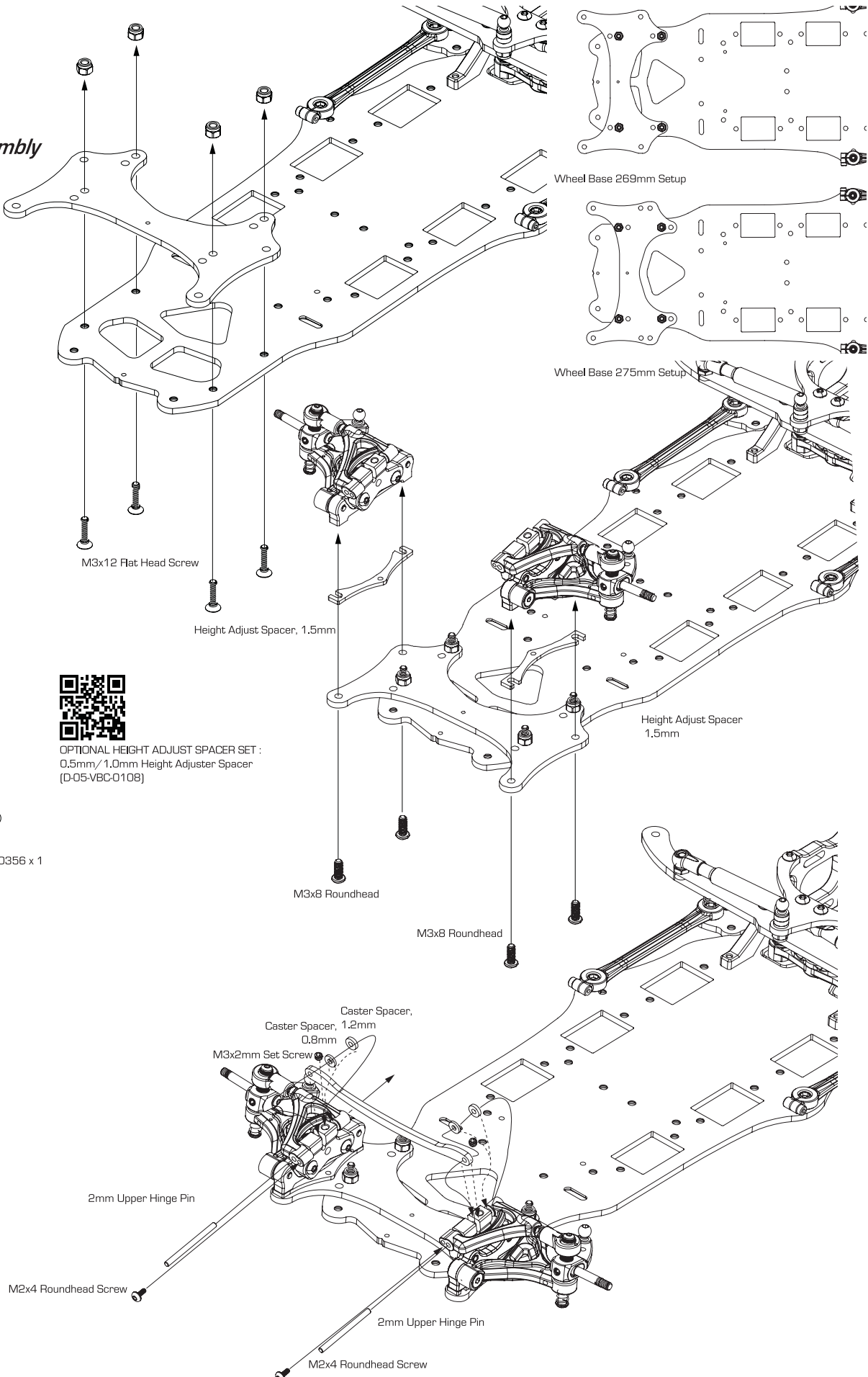
M2x4 Roundhead Screw C-02-SC-R0204 x 2
