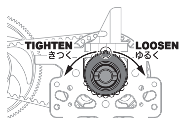
LOWER DIFF POSITION デフ位置 低
